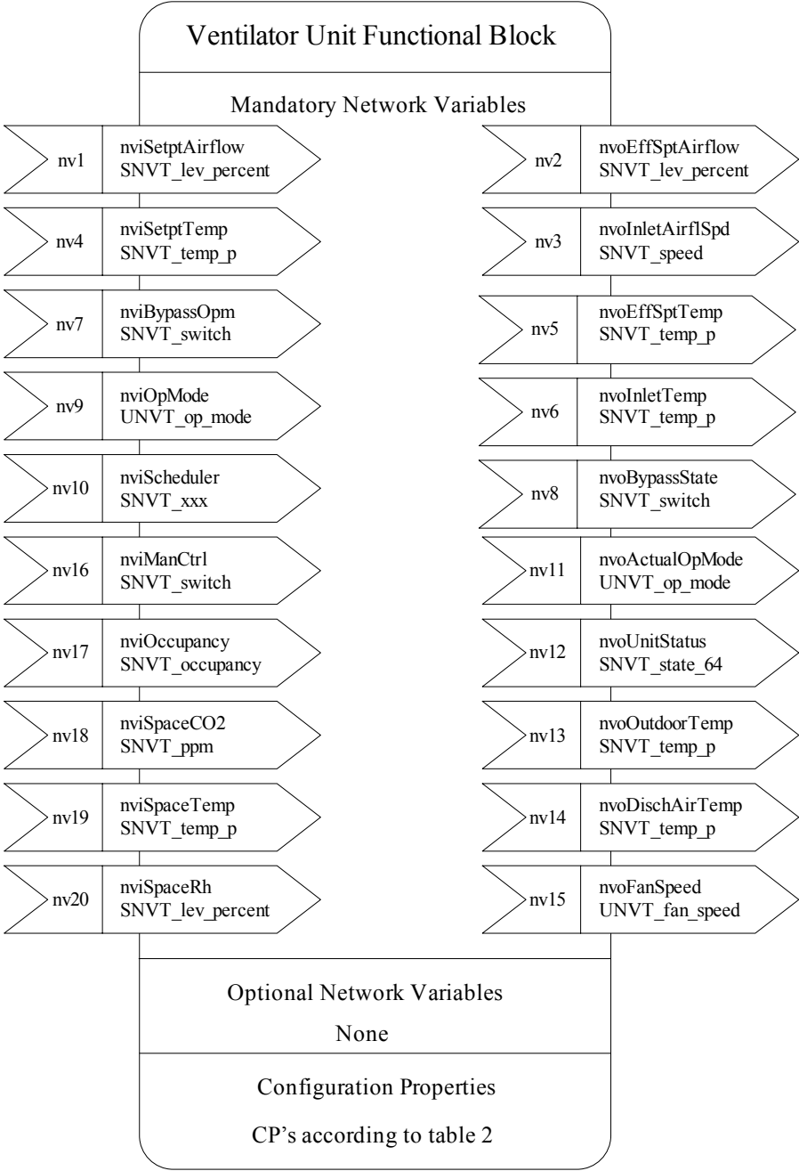
Figure 2 Functional-Block Details
